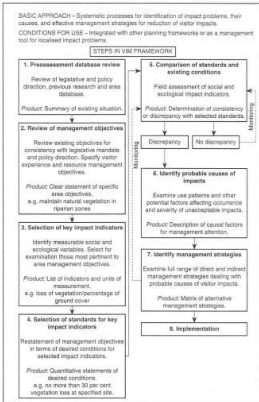
Figure 6.2 Visitor Impact Management framework
